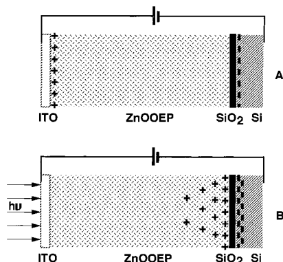
FIGURE 11. Schematic diagram of the operational principles for charge storage in a photoconductive medium (A) in the dark and (B) with irradiation. Reprinted with permission from ref 8. Copyright 1996 The Electrochemical Society.
